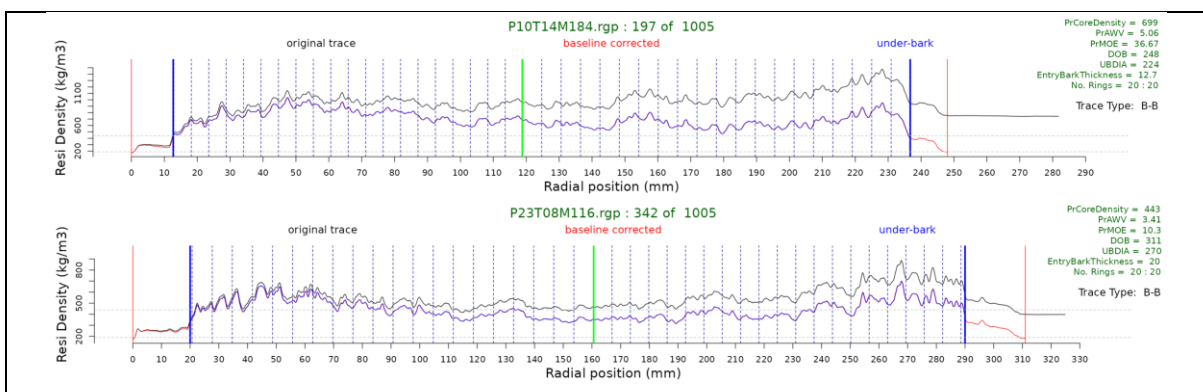
Figure 120: Two examples of typical Resi traces are presented, where the Resi needle has entered from the left (north) and exited on the right (south).
